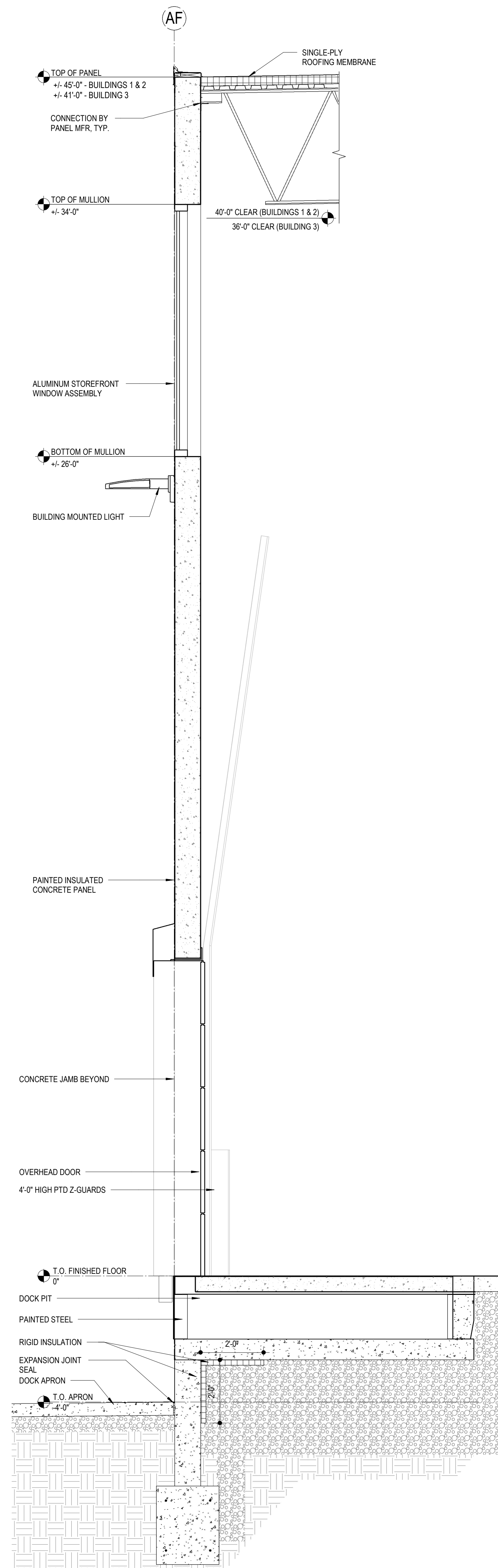
1 TYPICAL WALL SECTION AT LOADING DOCK 1/2" = 1'-0"
